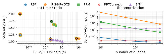
Fig. 4. Shelf+IIWA cross-algorithm trade-off. Black rings mark first full-success points; panel (b) uses Table III online-only timing and reusable-build terms where applicable.
