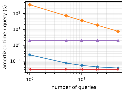
✕ RRTConnect ▲ BIT* (b) amortization
