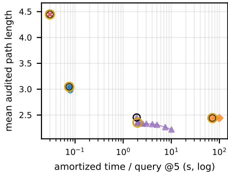
● RBF ◆ IRIS-NP+GCS (a) time / path
