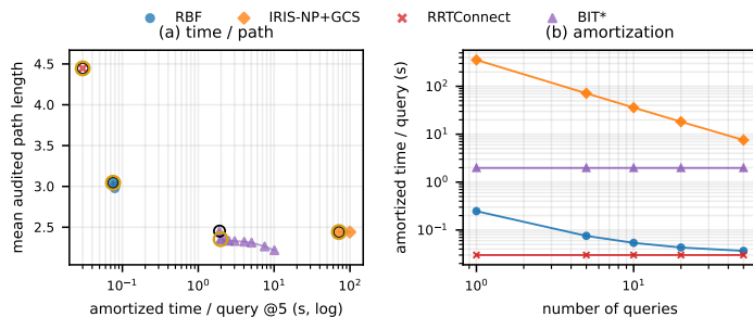
Fig. 4. Shelf+IIWA cross-algorithm trade-off. Panel (a) shows full-success amortized time-path points; black rings mark first full-success points; panel (b) shows Table III amortization.
