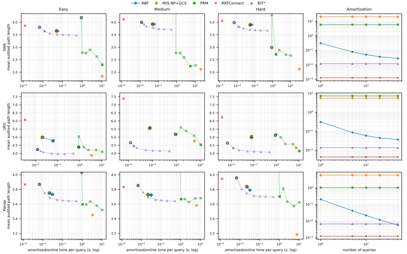
Fig. 5. Saved-catalog random-scene trade-off. Rows separate IIWA, UR5, and Panda; columns show easy, medium, hard, and per-robot query-count amortization. Blue curves are RBF budget sweeps on the saved v6 multi-query catalog. PRM and BIT* are saved-catalog reruns with the same 0.01 rad final audit. The IRIS-NP+GCS table column restores the legacy random-scene contextual result. Only 100% success-rate points are plotted; black rings mark the first full-success point on each curve and gold rings mark the tabulated trade-off point. Context rows for non-RBF reusable planners are shown when available under the same saved-scene protocol.
