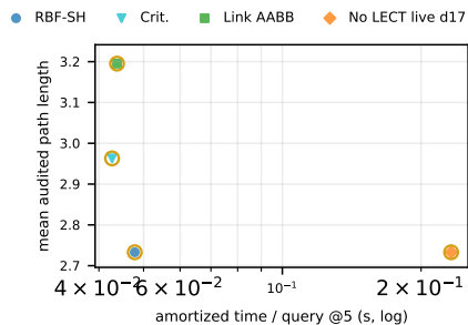
Fig. 3. Shelf+IIWA RBF ablation. Amortized time/query versus audited path length; only full-success points are shown; gold rings mark Table II rows.
