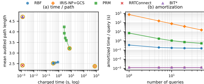
Fig. 4. Shelf+IIWA cross-algorithm trade-off. Panel (a) shows time-path trade-off; panel (b) shows Table III amortization.
