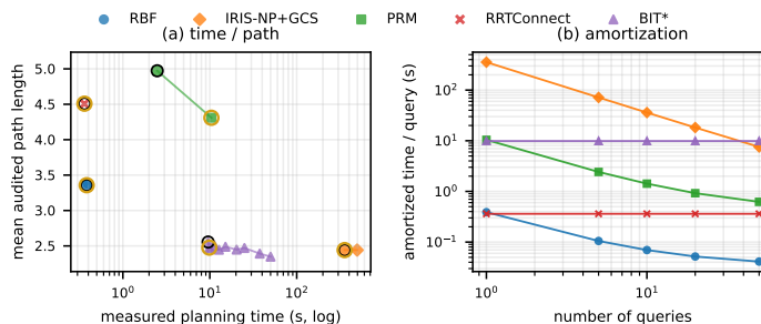
Fig. 4. Shelf+IIWA cross-algorithm trade-off. Panel (a) shows only full-success time-path points; black rings mark first full-success points; panel (b) shows Table III amortization.
