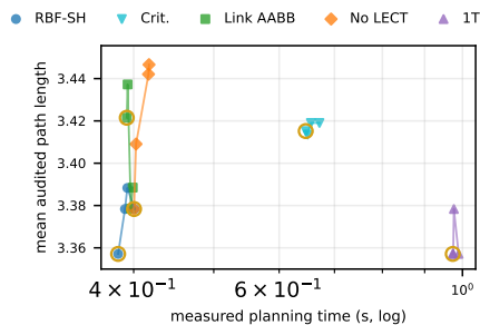
Fig. 3. Shelf+IIWA RBF ablation. Time versus audited path length; only full-success points are shown; gold rings mark Table II rows.
