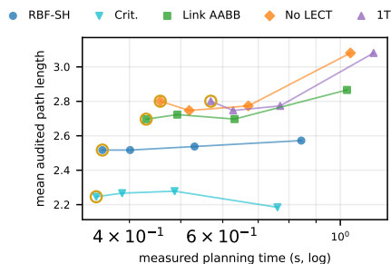
Fig. 3. Shelf+IIWA RBF ablation. Time versus audited path length; rings mark Table II rows.
