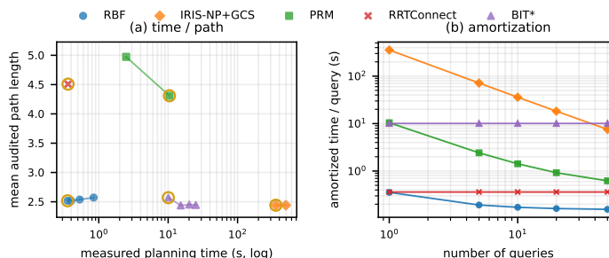
Fig. 4. Shelf+IIWA cross-algorithm trade-off. Panel (a) shows time-path trade-off; panel (b) shows Table III amortization.
