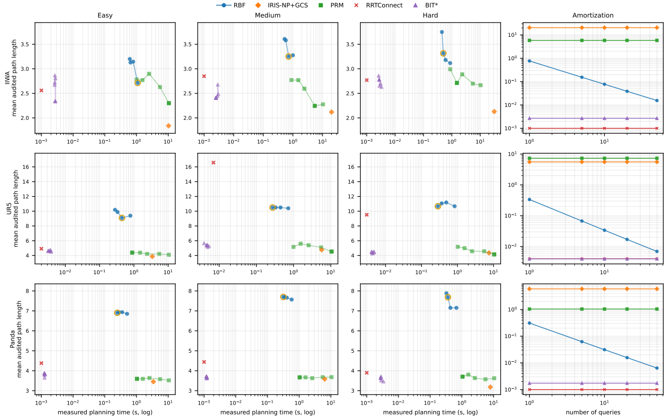
Fig. 5. Saved-catalog random-scene trade-off. Rows separate IIWA, UR5, and Panda; columns show easy, medium, hard, and per-robot query-count amortization. Blue curves are current RBF budget sweeps on the saved v5 catalog. PRM, RRTConnect, and BIT* are rerun on the same catalog with the same 0.01 rad final audit, while IRIS-NP+GCS is imported from the old balanced random-scene common-rule artifact as protocol context.
