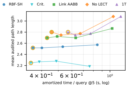
Fig. 3. Shelf+IIWA RBF ablation. Amortized time/query versus audited path length; only full-success points are shown; gold rings mark Table II rows.
