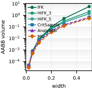
Volume objective (certified lower; samples higher)
