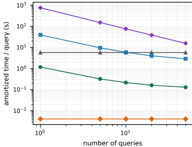
Query amortization
