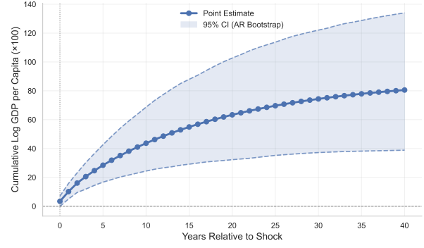
B. Cumulative Response to Permanent Shock
