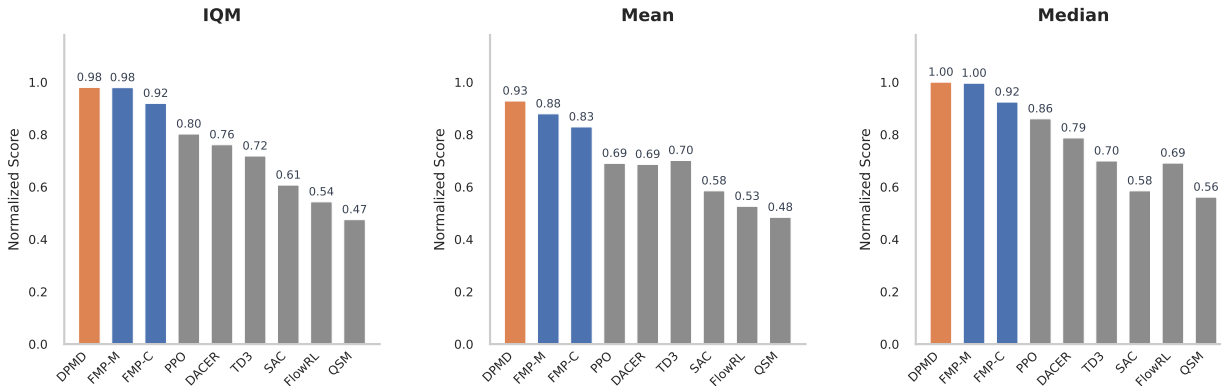
Figure 1: Aggregated normalized best evaluation returns across 10 MuJoCo tasks. For each task, the return is normalized to [0, 1] using the minimum and maximum returns across all methods. The interquartile mean (IQM) excludes the top and bottom two task scores for each method to mitigate the effect of outliers.
