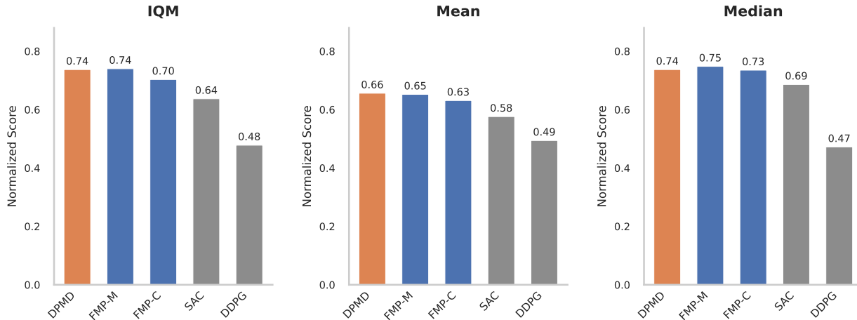
Figure 2: Aggregated normalized best evaluation returns across 8 DeepMind Control Suite tasks. For each task, the return is normalized to [0, 1] by dividing by 1000.
