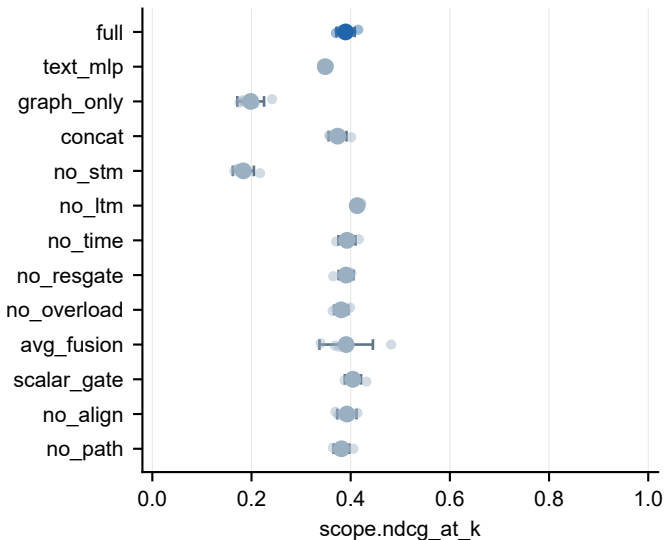
SIM-Energy | synthetic; mean \pm sample SD across training seeds
