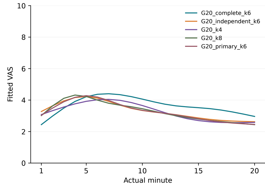
D Approximate covariance conditioning
