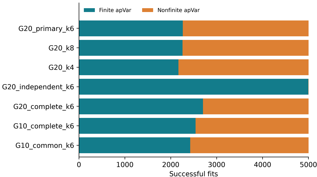
C apVar records per 5,000-fit cell
