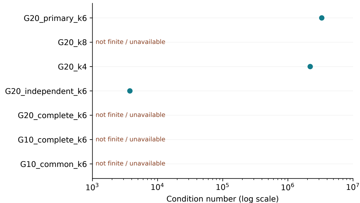
D Approximate covariance conditioning
