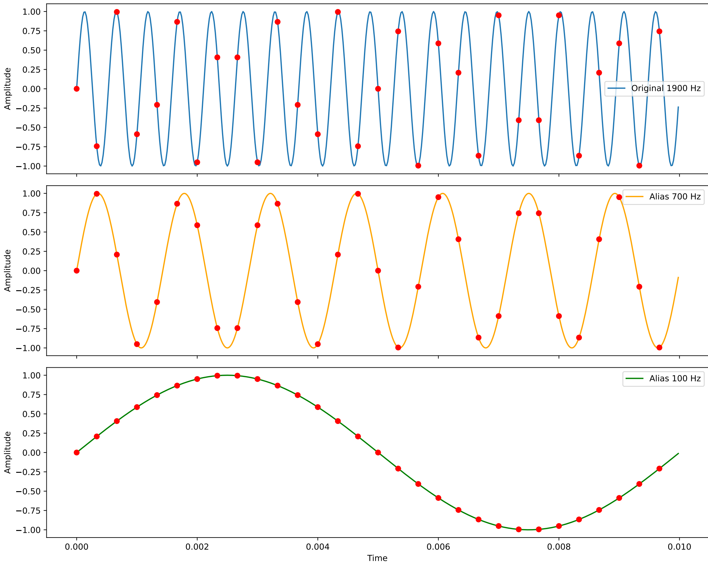
Aliasing Demonstration: Same Sample Points for Different Frequencies
