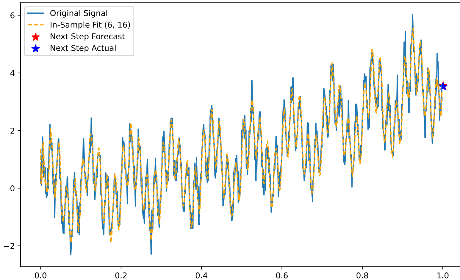
ARMA(6, 16) Model: Fit & Forecast
