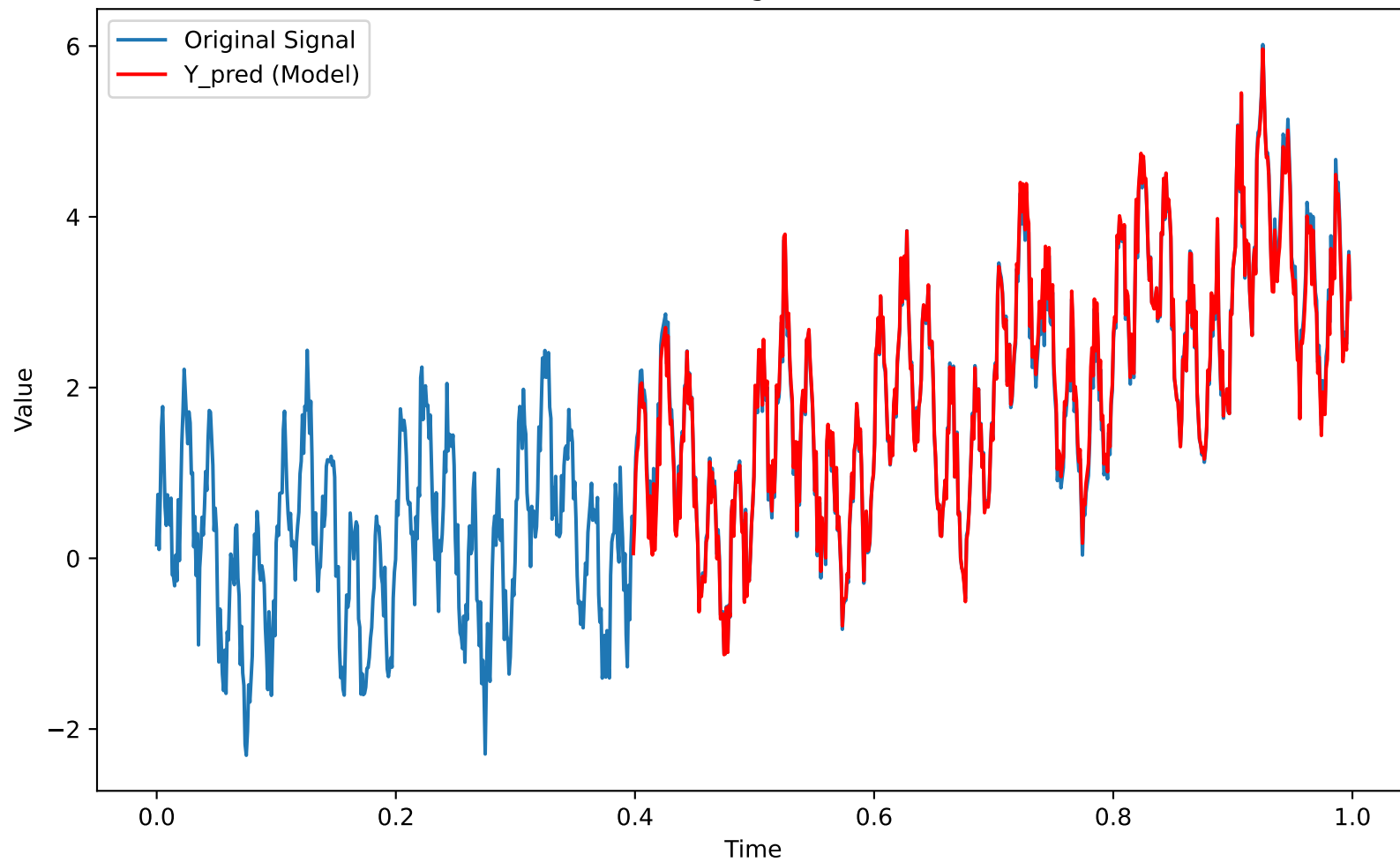
MA(200) Model: Signal vs Predictions
