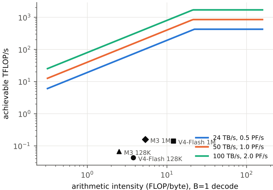
Decode roofline: workloads vs Fabrik configurations
