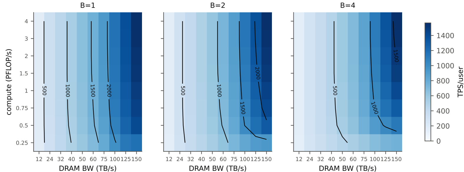
MiniMax M3 fp8 @128K: TPS/user over bandwidth x compute
