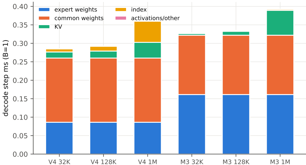
Latency decomposition (V4 on 50 TB/s; M3 on 100 TB/s)
