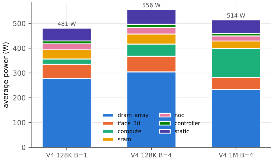
Power decomposition, Fabrik 50 TB/s / 1 PF
