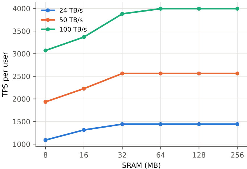
SRAM sensitivity (V4-Flash @128K, B=1)
