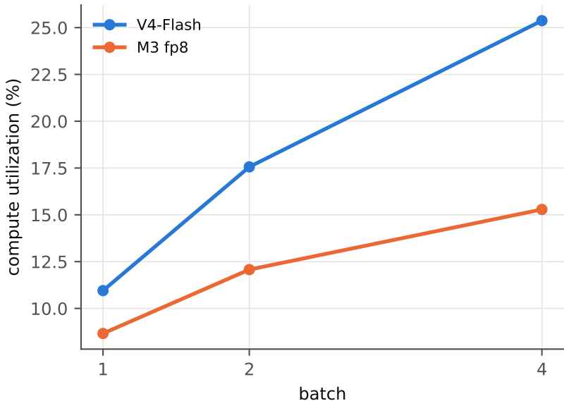
Compute utilization vs batch (50 TB/s, 1 PF)
