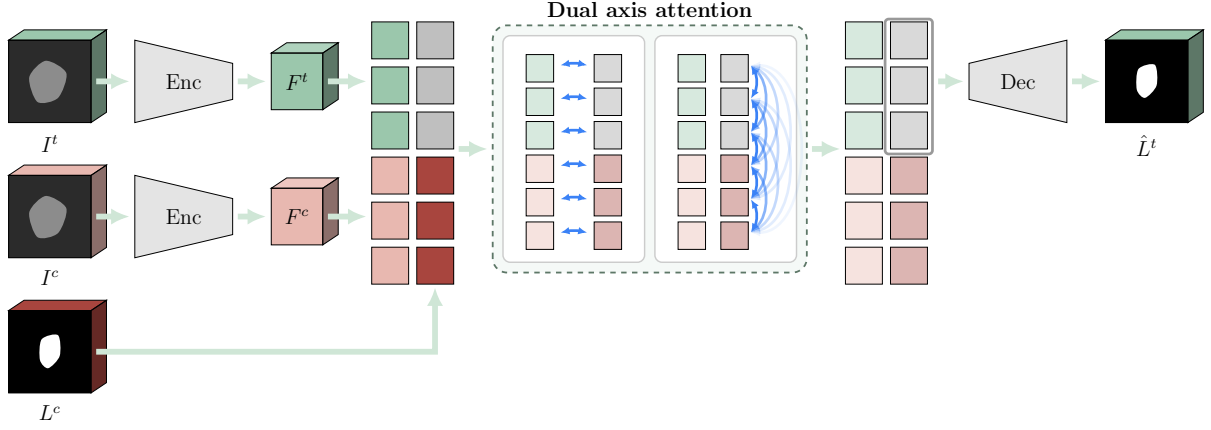
Figure 1: Overview of the model at one cascade level. Target and context images pass through a shared encoder; image and label tokens are processed by dual attention; a decoder produces the target mask.
