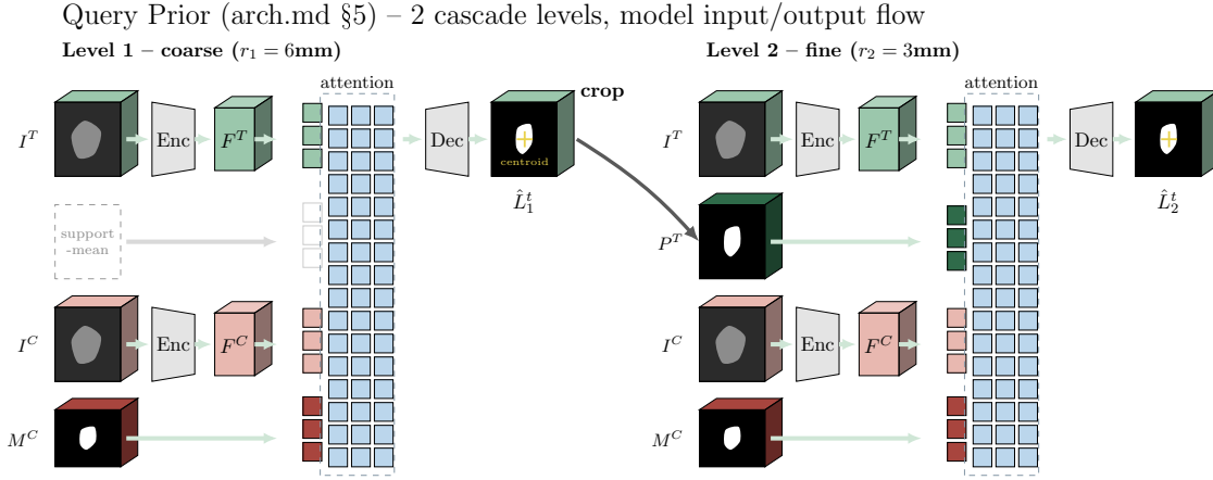
level 1: target's 2nd lane = support-mean (no real input) \rightarrow level 2: target's 2nd lane = P^T , a REAL cube (crop of \hat{L}_1^t ) – same lane the context mask always occupies
