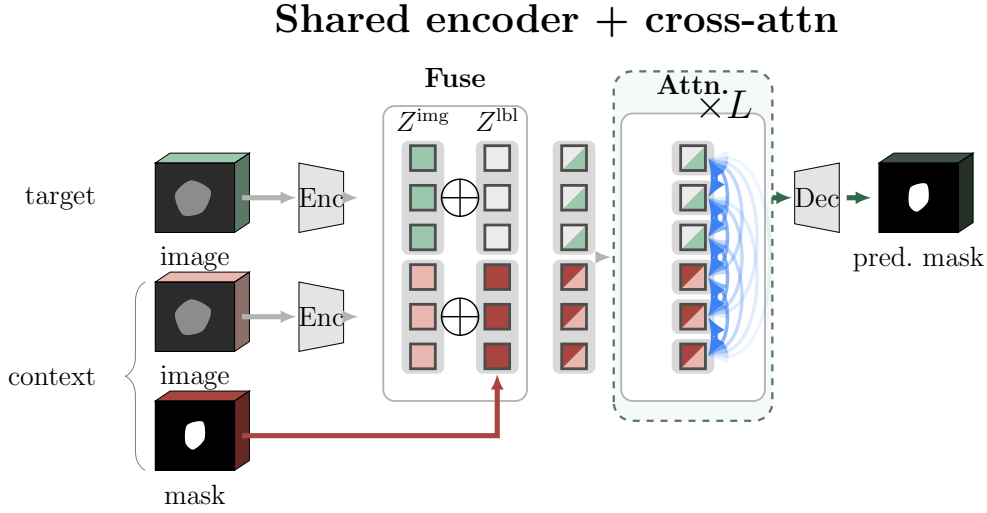
Figure 2: Two ways of coupling target and context, shown for one context volume ( K=1 ) and three of its N tokens. Top: Medverse feeds the target image, and the context image and mask concatenated as channels, into two separate U-Nets that exchange features through cross-attention at several stages (blue arrows). Bottom: the shared-encoder design used in this thesis. Only images pass through the encoder. Label information is added to the encoded tokens afterwards, the tokens attend across cells and volumes for L layers, and a shared decoder produces the mask. ?? shows the two ways of adding label information that we compare.
