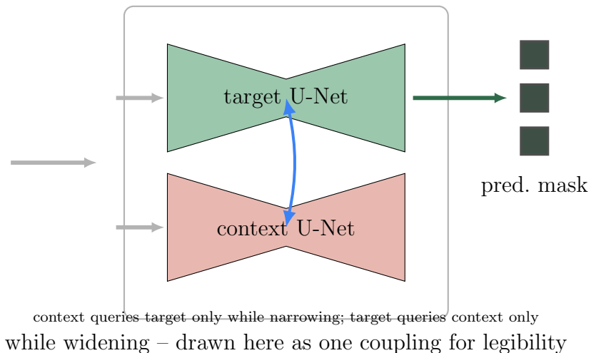
Dual U-Net (separate weights)
