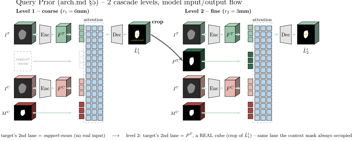
Figure 3: Query image prior across two cascade levels, with the full model input/output flow. At level 1 the target has no real prior yet (dashed support-mean placeholder); at level 2 the target's second lane is a real crop of level 1's own prediction \hat{L}_1^t – the same lane the context mask always occupies.
