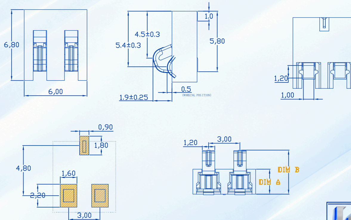
RECOMMENDED PCB LAYOUT TOP VIEW (.XX±0.05)
