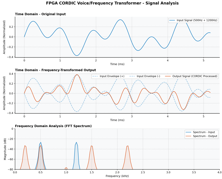
Fig. 6. Time-domain and Frequency-domain (FFT) analysis of the CORDIC DSB-SC pitch shifter.
