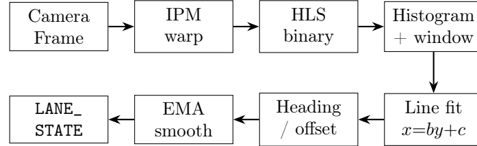
Figure 14: Lane detection pipeline
