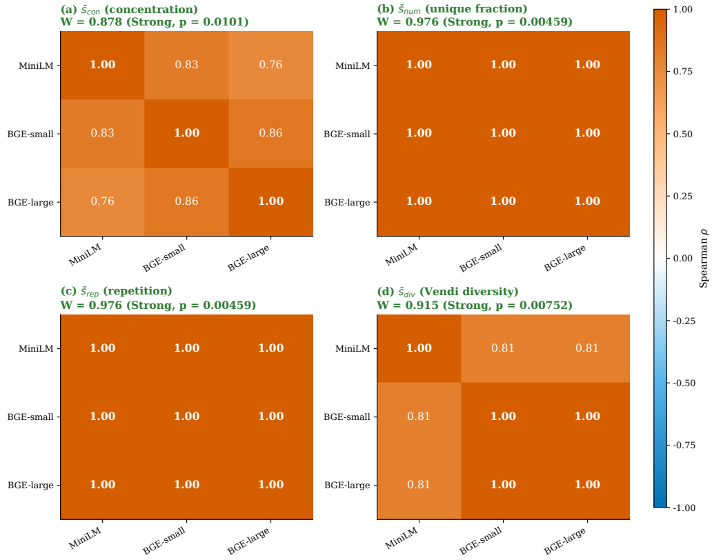
Figure 2: Figure 4 · Cross-model stability · pairwise Spearman \rho (3 sentence-transformers) · within-paradigm ranking agreement
