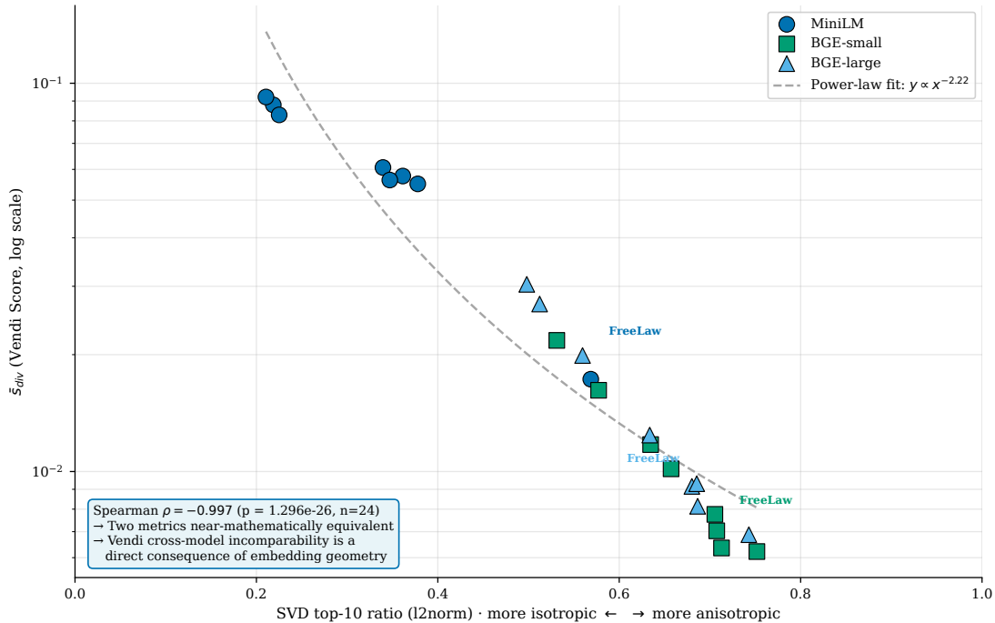
Figure 3: Figure 2 · Vendi-SVD triangulation (sentence-transformers only, n=24 , \rho \approx -0.997 )
