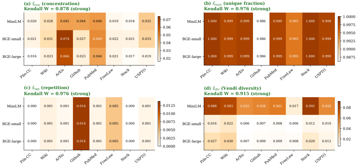
Figure 1: Figure 3 · \bar{s} four components \times 8 domains \times 3 sentence-transformers models · within-paradigm ranking stability
