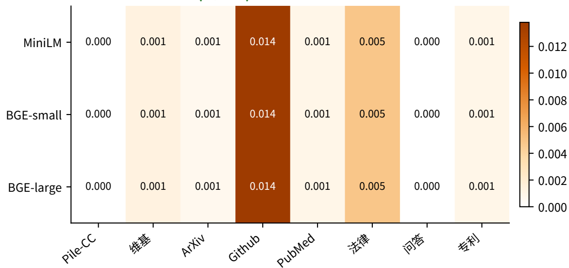
(c) \bar{s}_{rep} (重复度) Kendall W = 1.000 (强一致)
