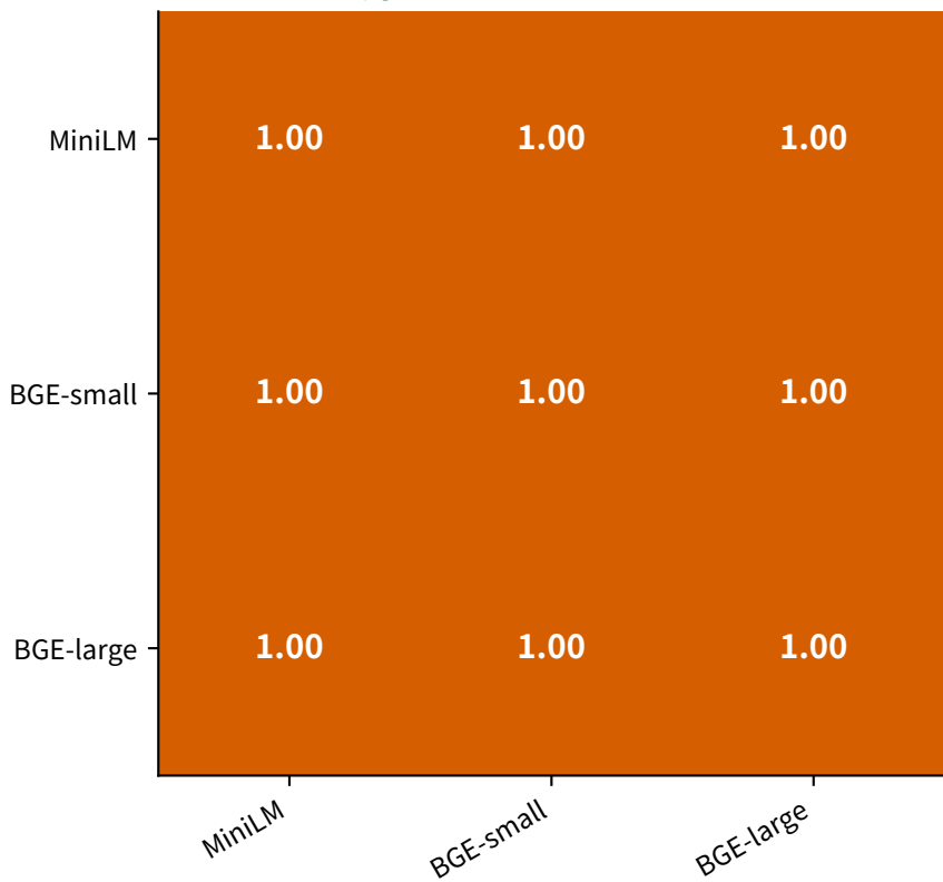
(c) \bar{s}_{rep} (重复度) W = 1.000 (强, p = 0.00377)
