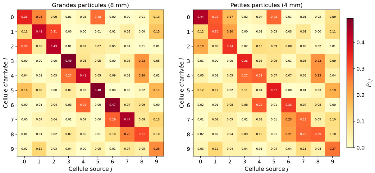
FIGURE 21 – Matrices de transition du découpage physique (10 cellules, configuration : nlt = 2 , start = 1,57 s, step = \tau = 1,57 s, dt = 8 pas)
