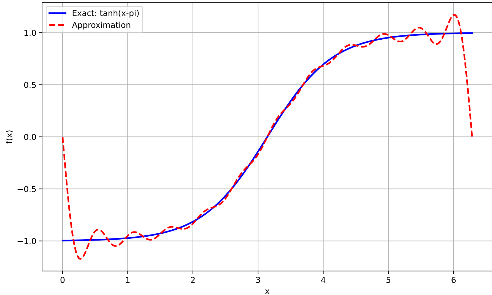
Least Squares Approximation
