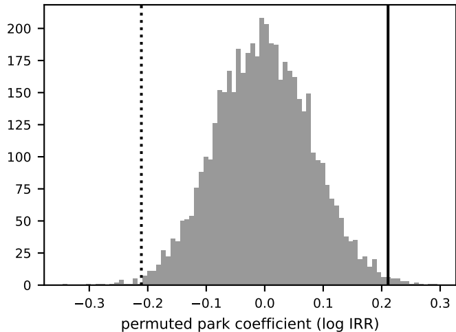
Unrestricted label permutation (5,000)
