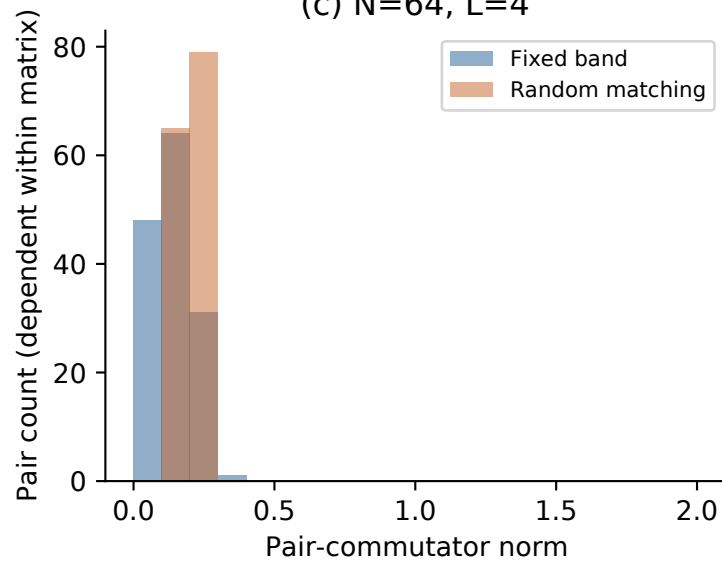
(c) N=64 , L=4
