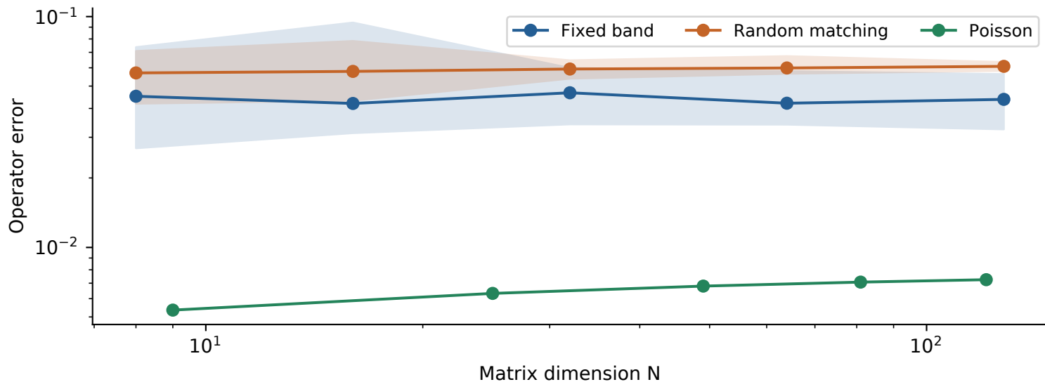
(a) Evolution time=1, r=4
