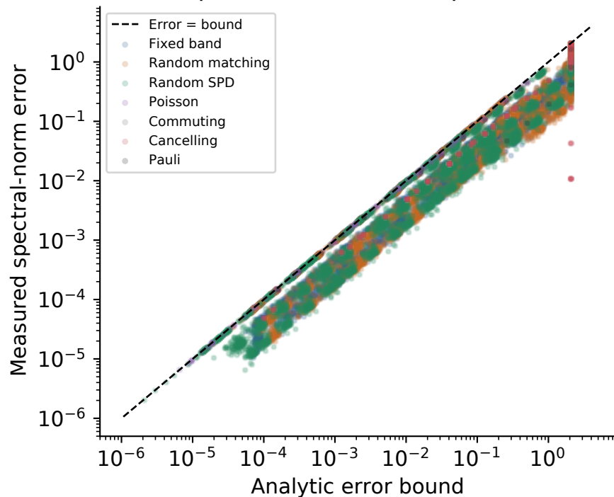
Operator error: all step sizes
