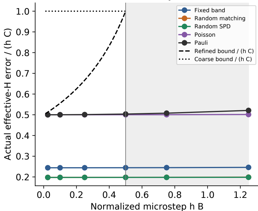
Matrix bound stated only for hB \leq 1/2
