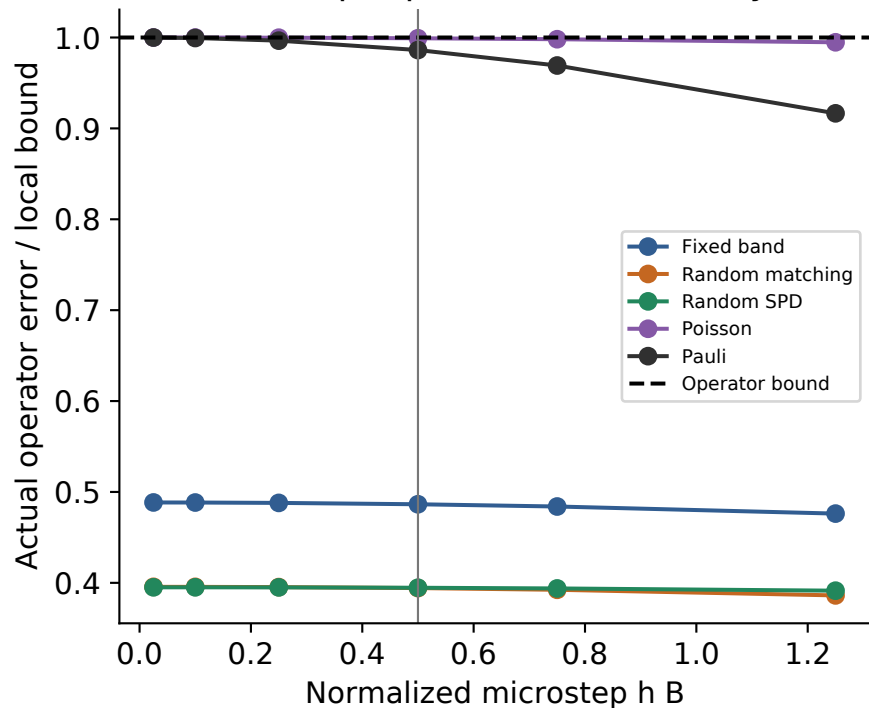
One microstep: operator bound always valid
