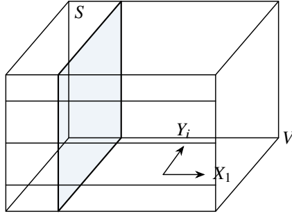
Coordinate slices and the transverse section S
