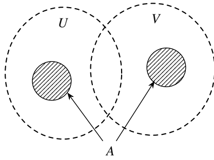
Figure A.4: A separation of A
