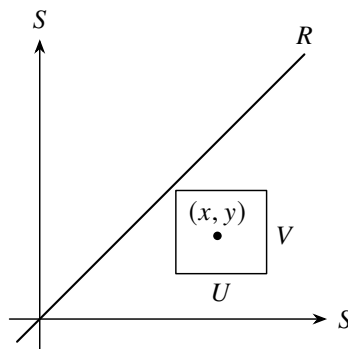
Figure A.8: The graph R of an equivalence relation and an open set U \times V disjoint from R (redrawn after [32])
