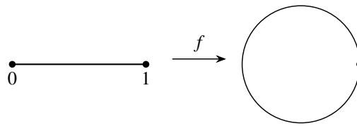
Figure A.6: The unit circle as a quotient of the unit interval (redrawn from [32])
