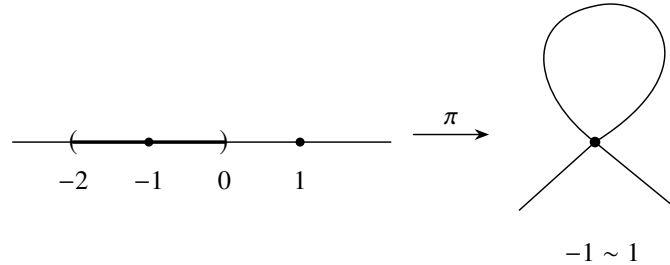
Figure A.7: A projection map that is not open (redrawn after [32])
