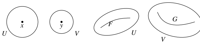
Figure A.3: The Hausdorff condition and normality, redrawn after [32]
