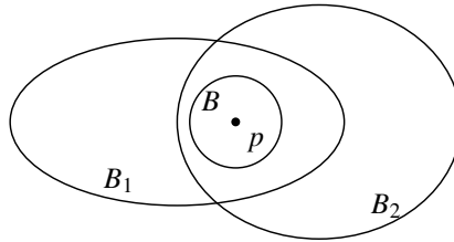
Figure A.2: The criterion for a basis, redrawn after [32]
