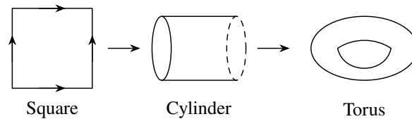
Figure A.5: Gluing the edges of a square (redrawn after [32])
