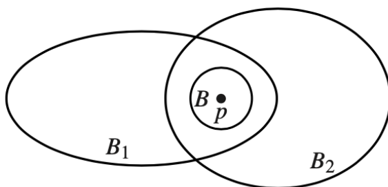
Figure A.2: The criterion for a basis, from [32]
