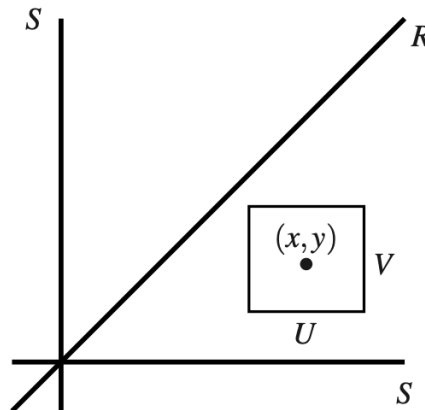
Figure A.8: The graph R of an equivalence relation and an open set U \times V disjoint from R (figure from [32])
