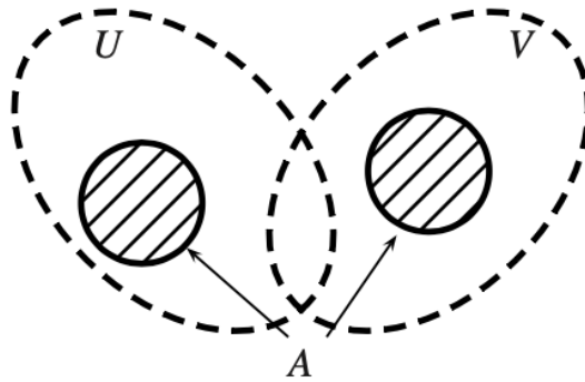
Figure A.4: A separation of A
