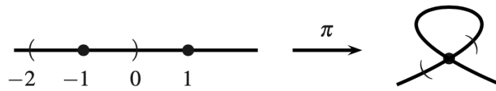
Figure A.7: A projection map that is not open (figure from [32])
