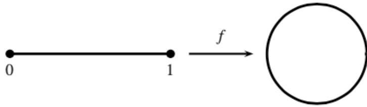
Figure A.6: The unit circle as a quotient of the unit interval (figure from [32])
