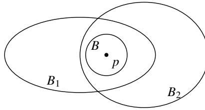
Figure A.2: The criterion for a basis, redrawn after [32]
