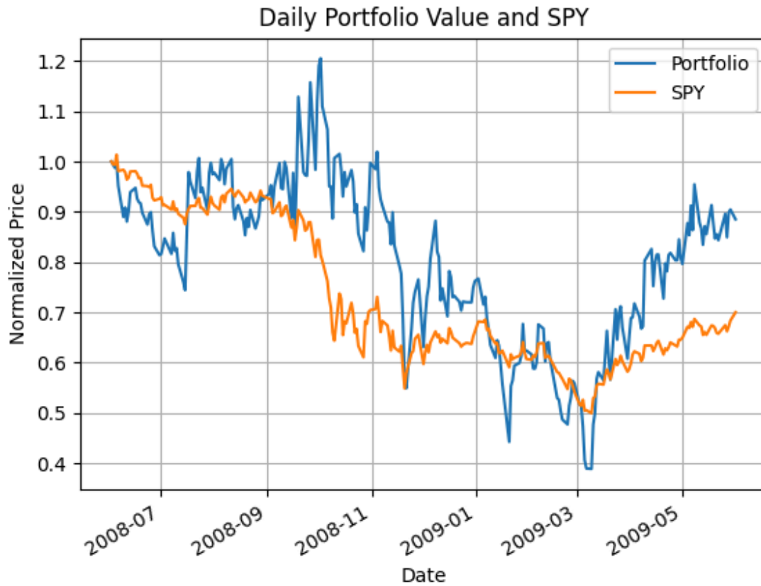
Figure 1- Comparison between Optimal Portfolio ('IBM', 'X', 'GLD', 'JPM') and SPY
