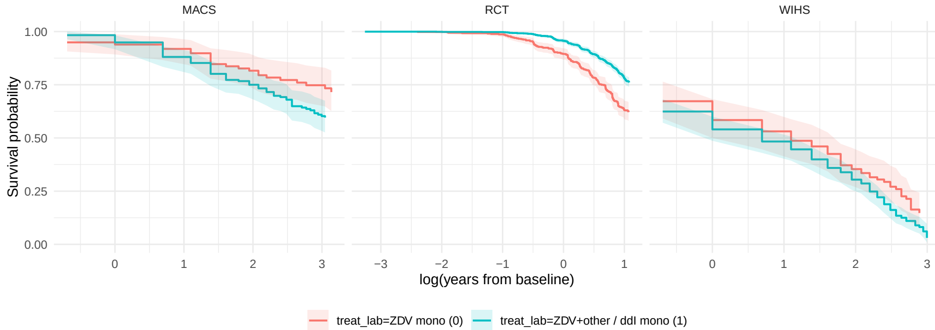
Kaplan–Meier survival by treatment, per dataset
