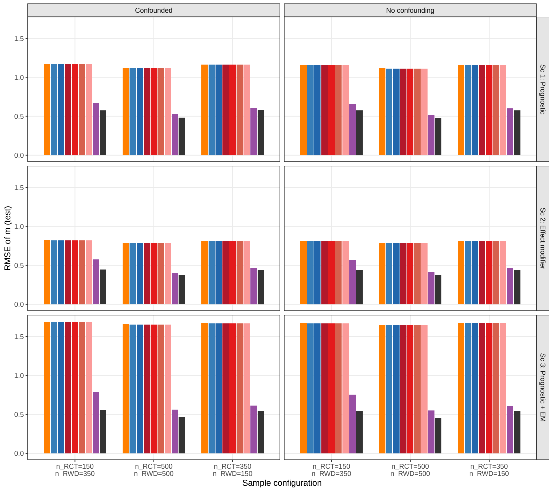
Prediction accuracy
