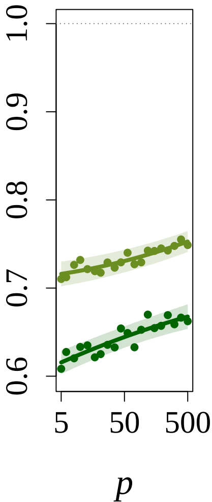
RMSE ratio (vs RCT-only)
