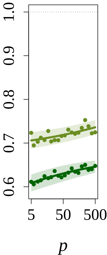
Posterior-variance ratio (vs RCT-only)
