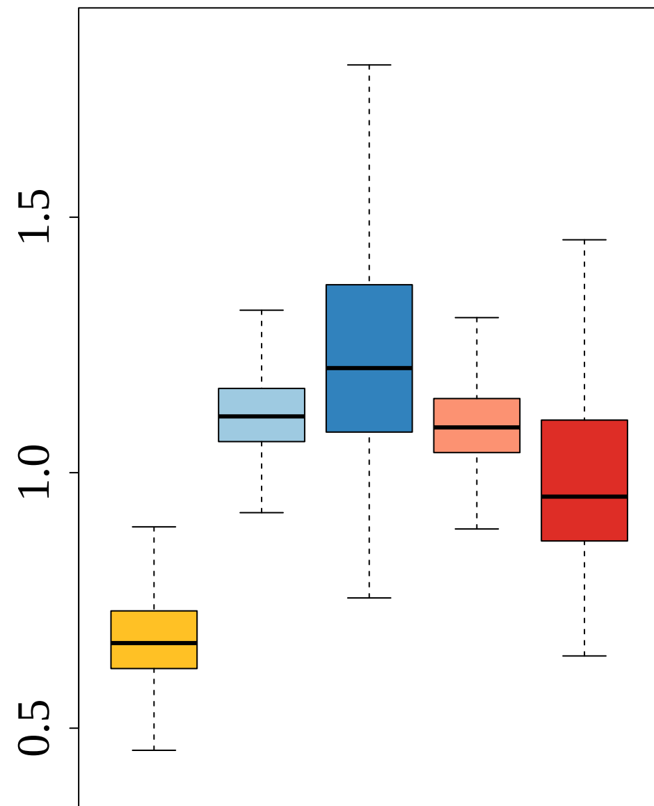
RMSE
