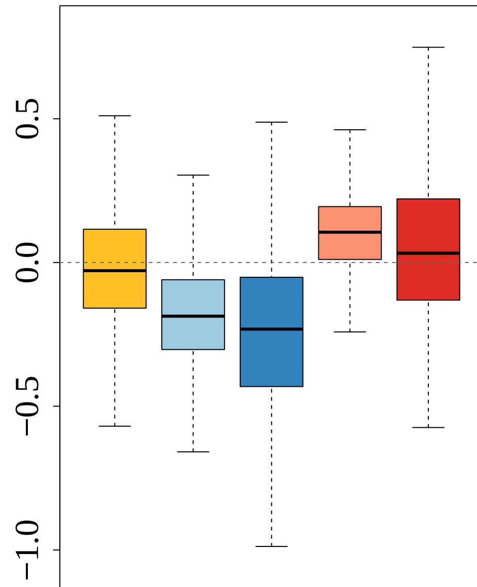
Bias
