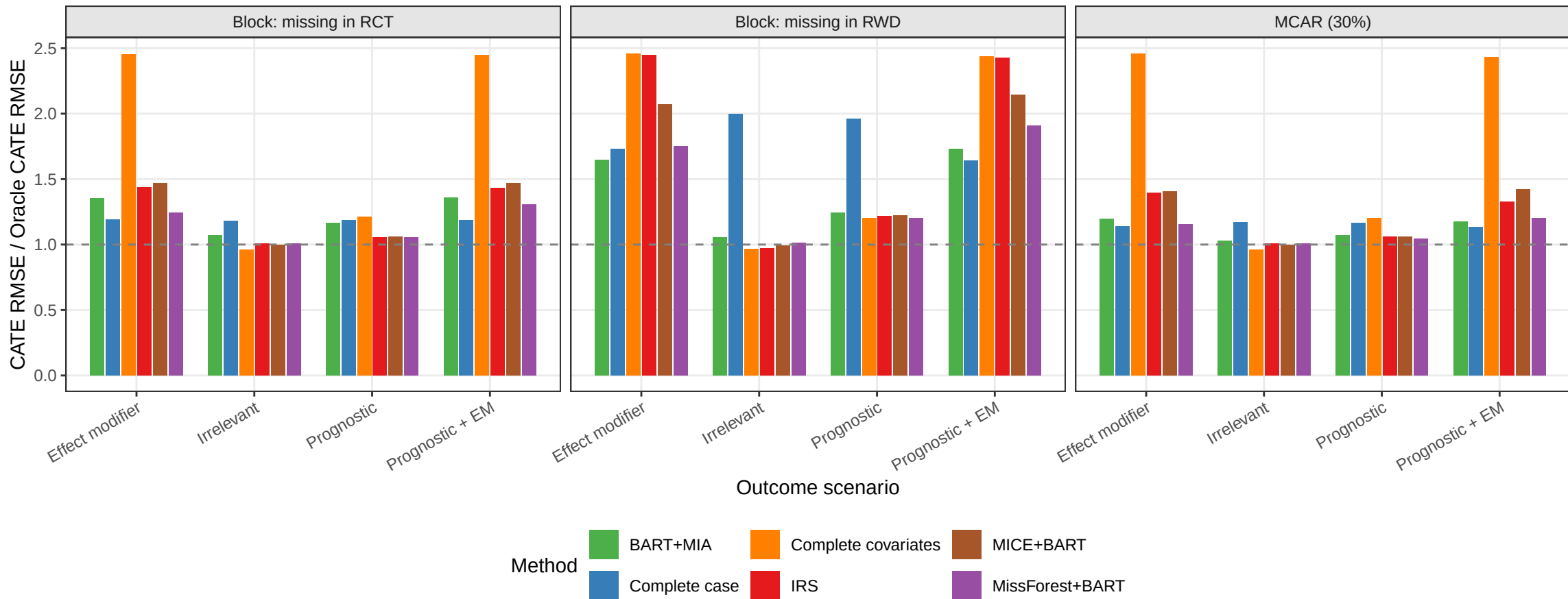
Relative CATE estimation efficiency
