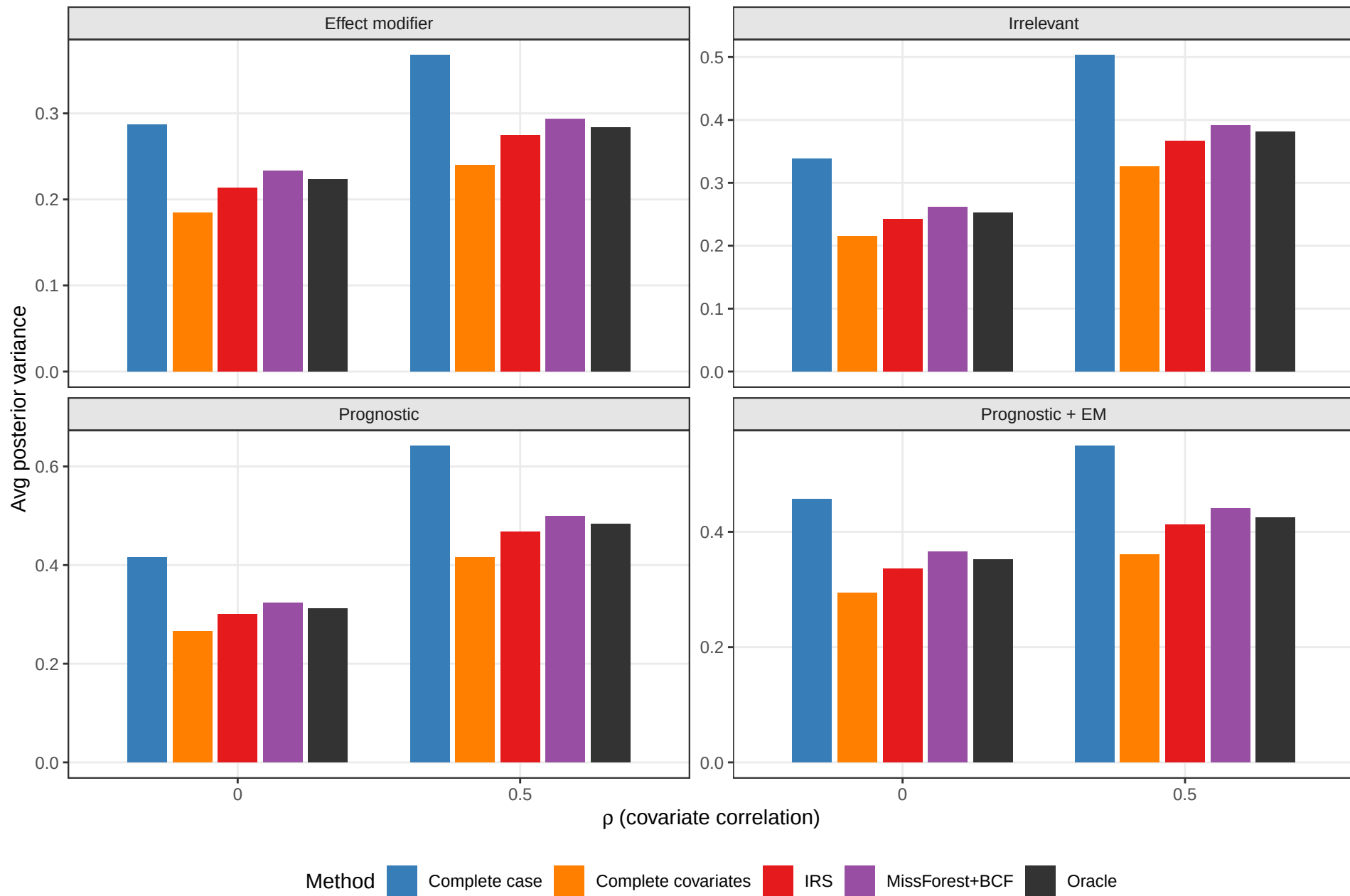
Average posterior variance of CATE
