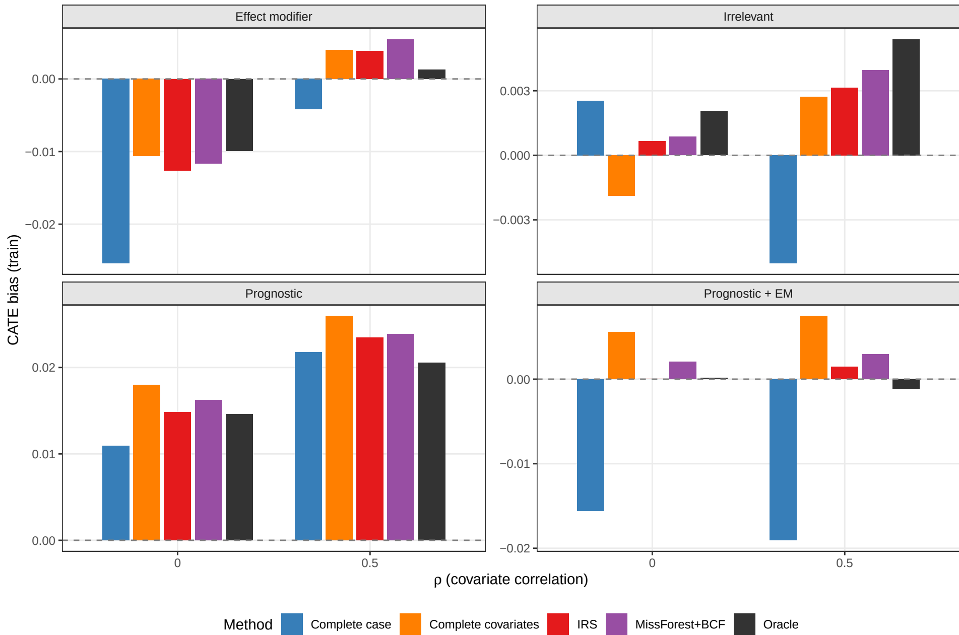
CATE estimation bias – training set
