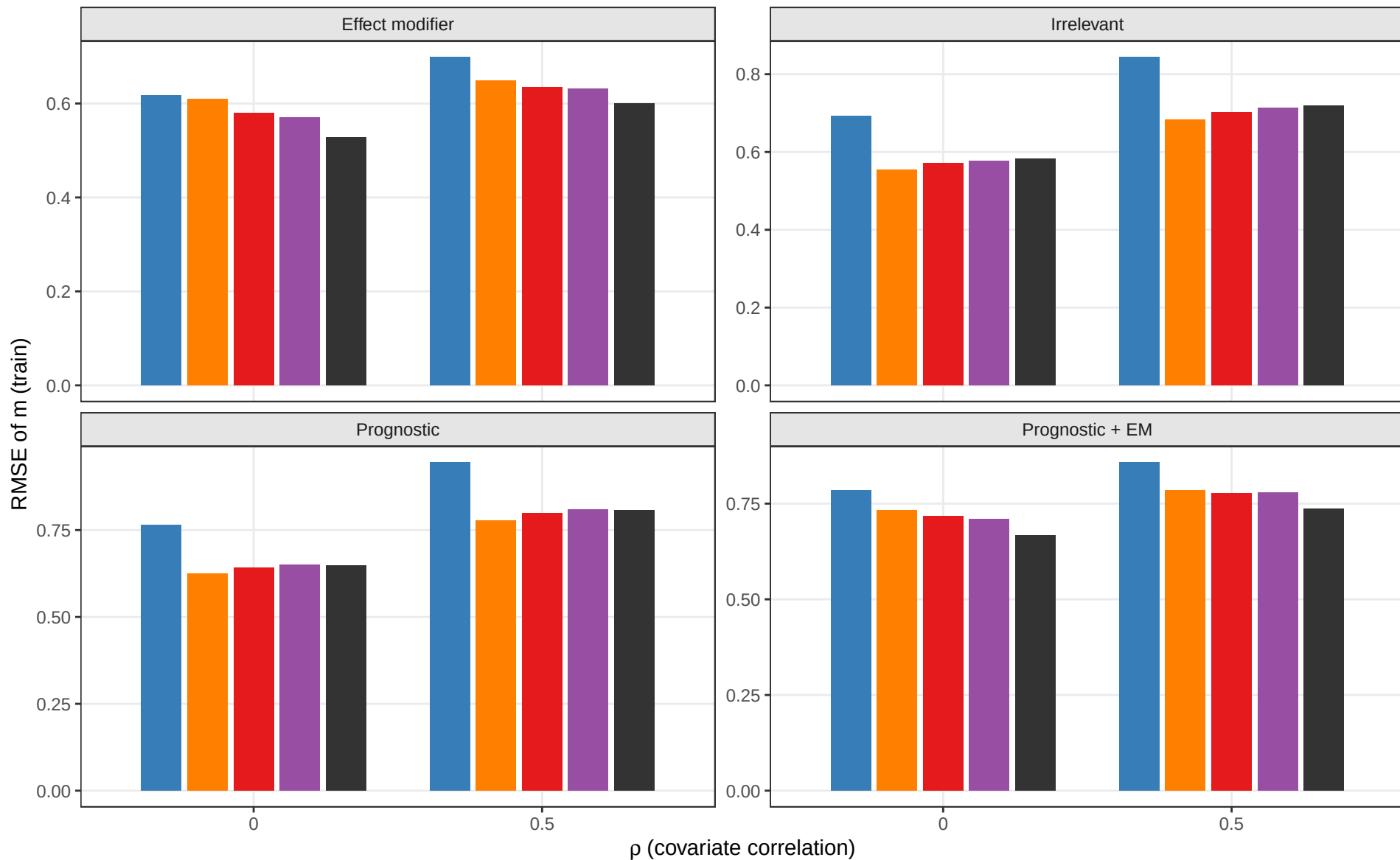
Prediction accuracy – training set
