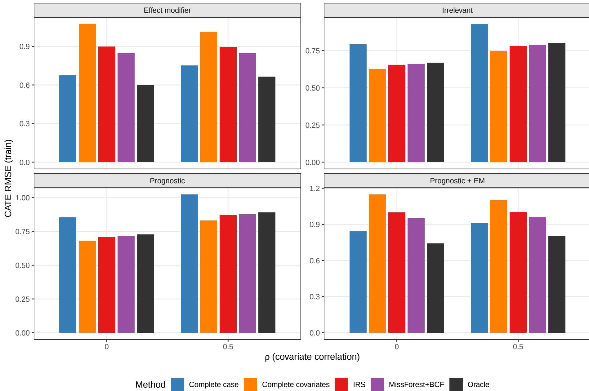
CATE estimation accuracy – training set
