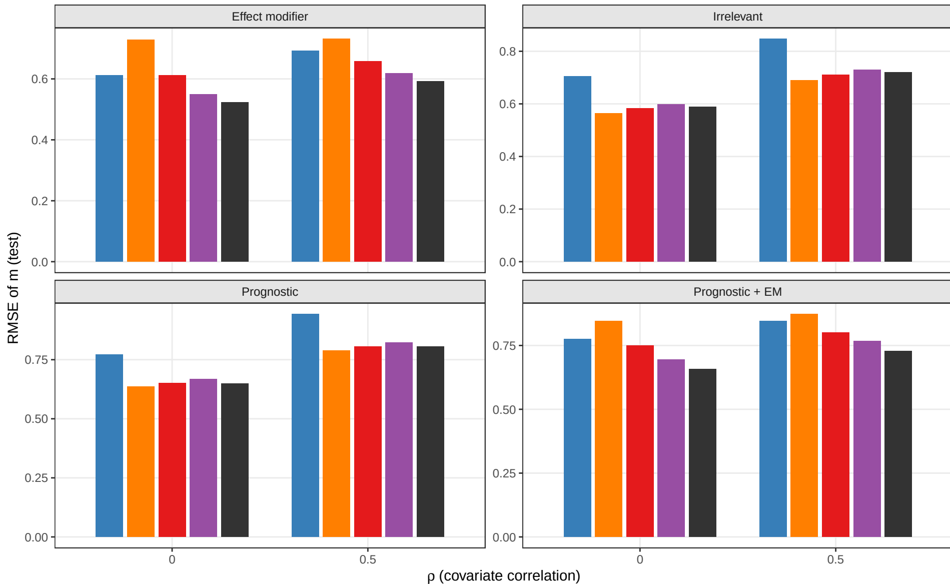
Prediction accuracy – test set
