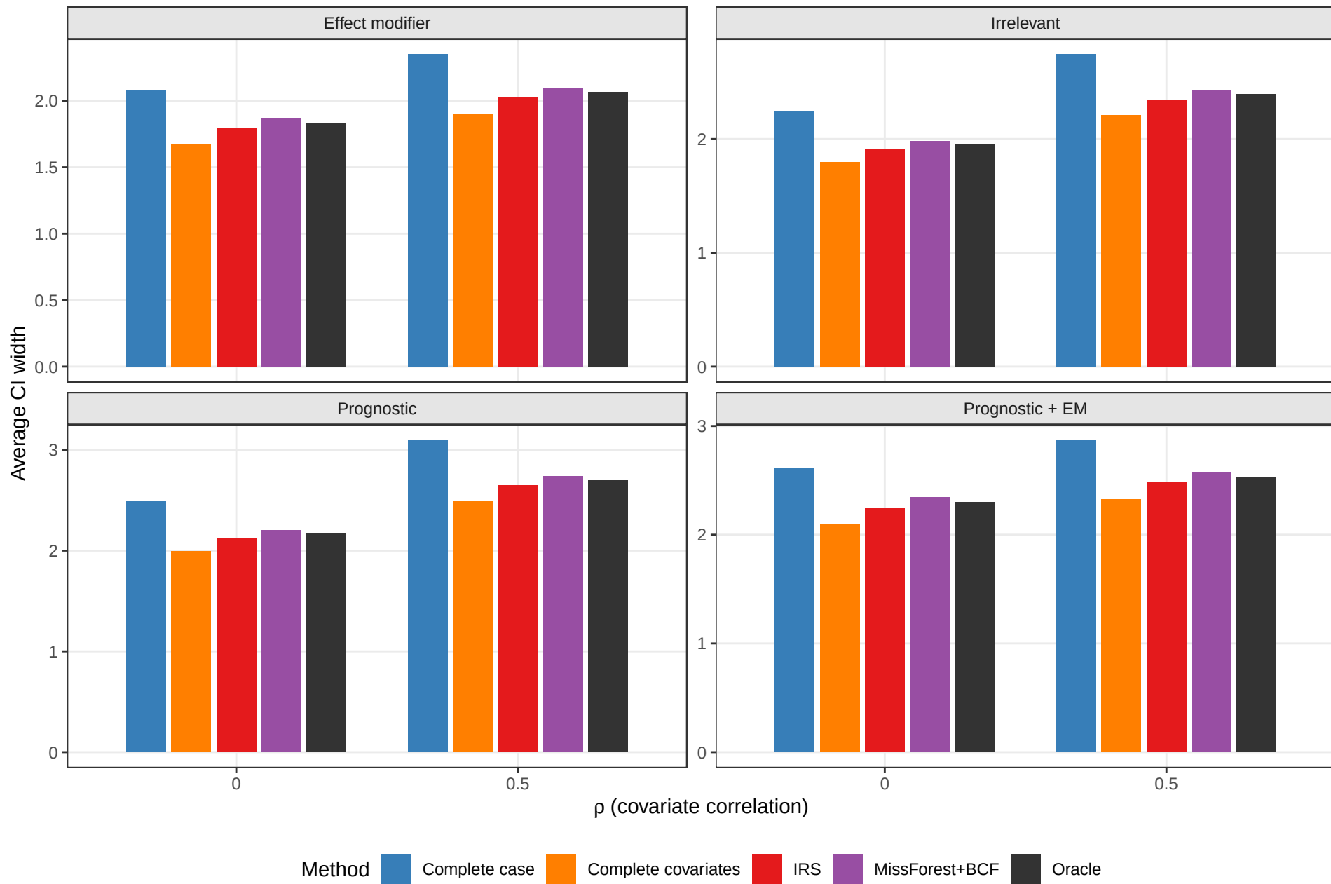
Credible interval width for CATE
