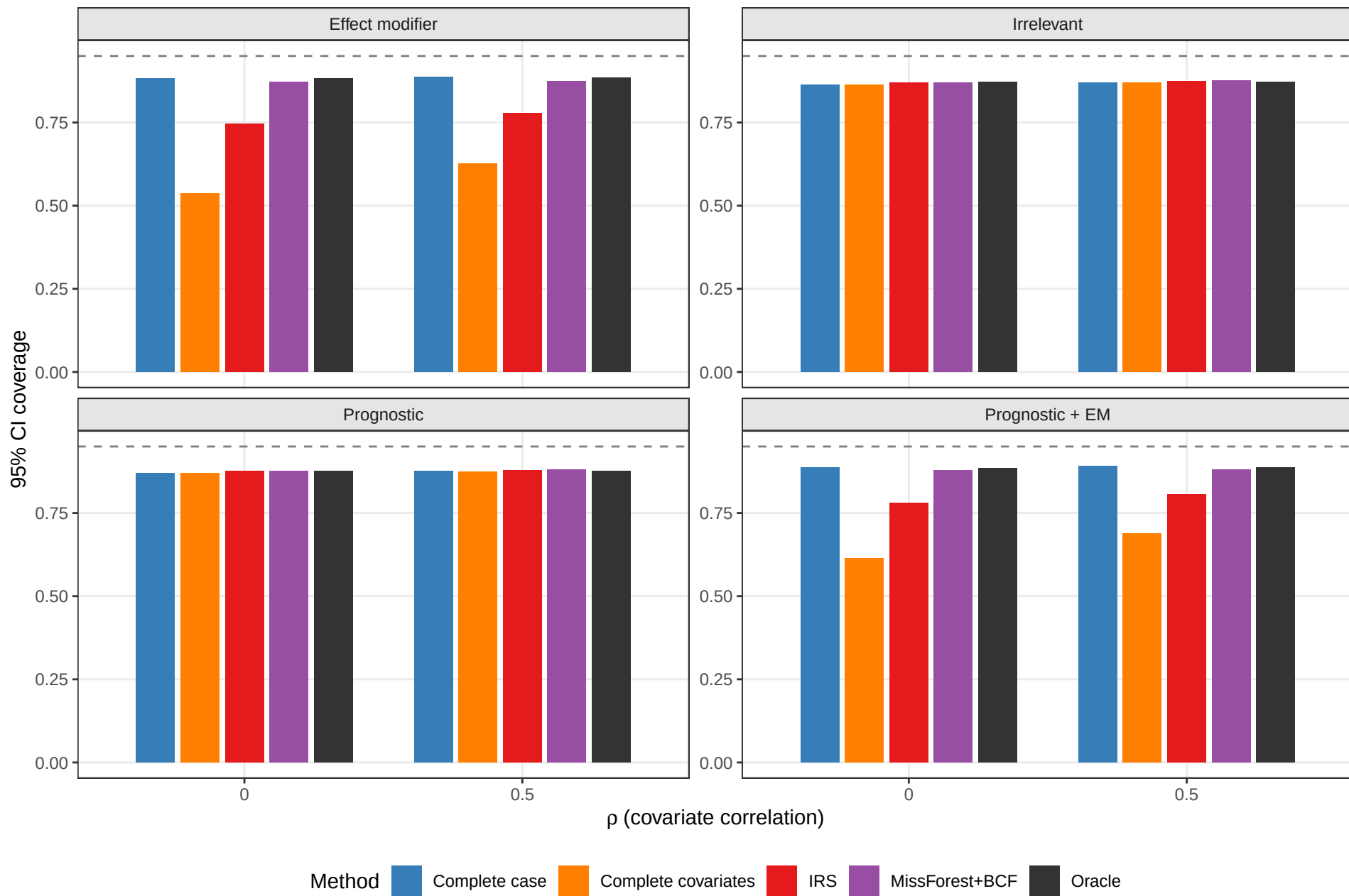
Credible interval coverage for CATE
