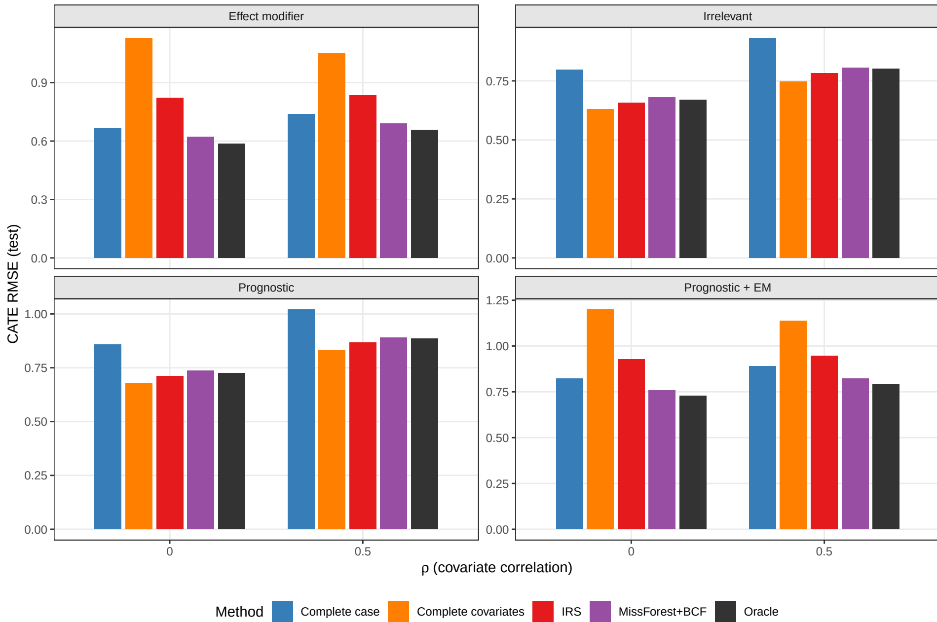
CATE estimation accuracy – test set
