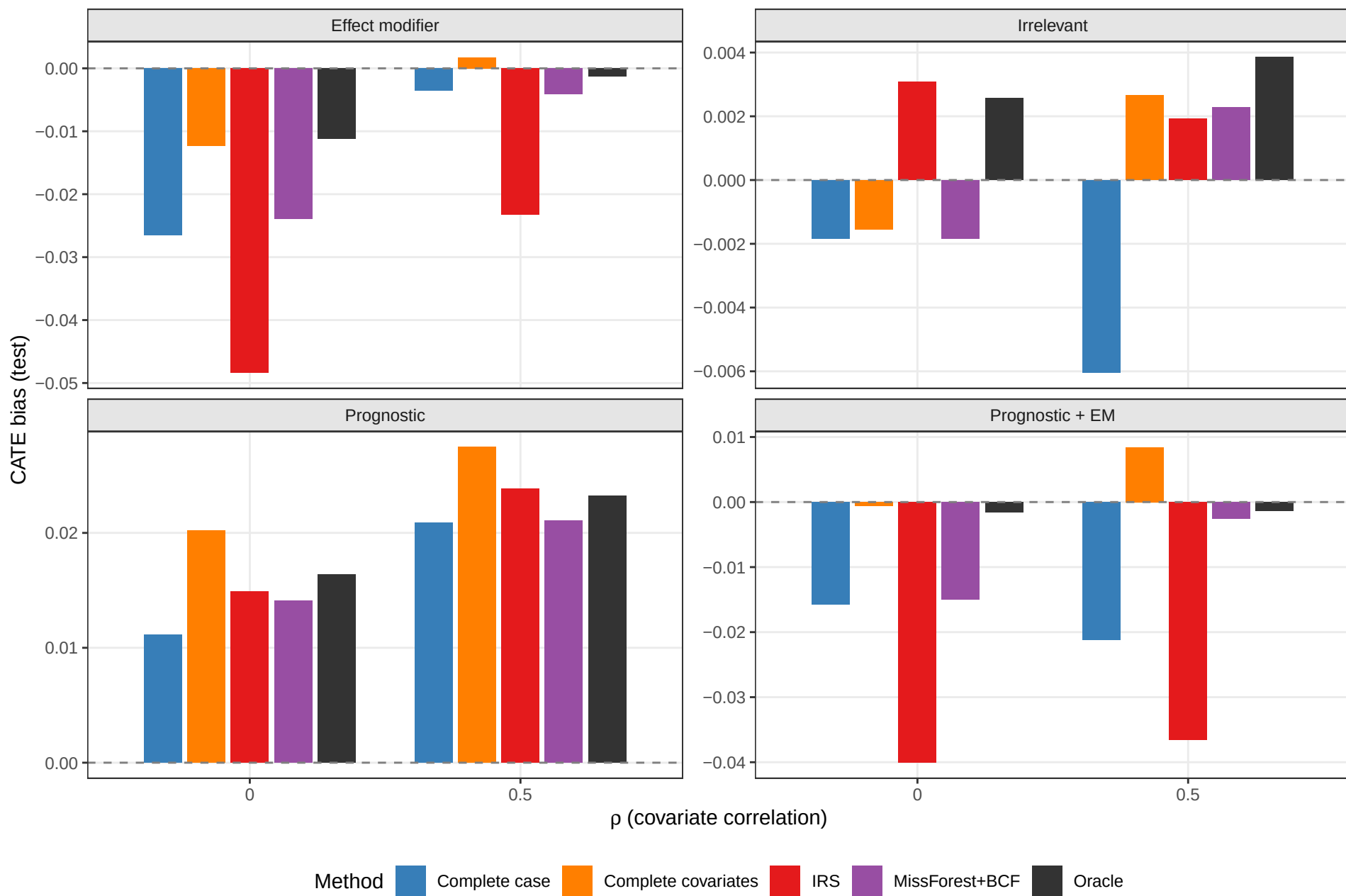
CATE estimation bias – test set
