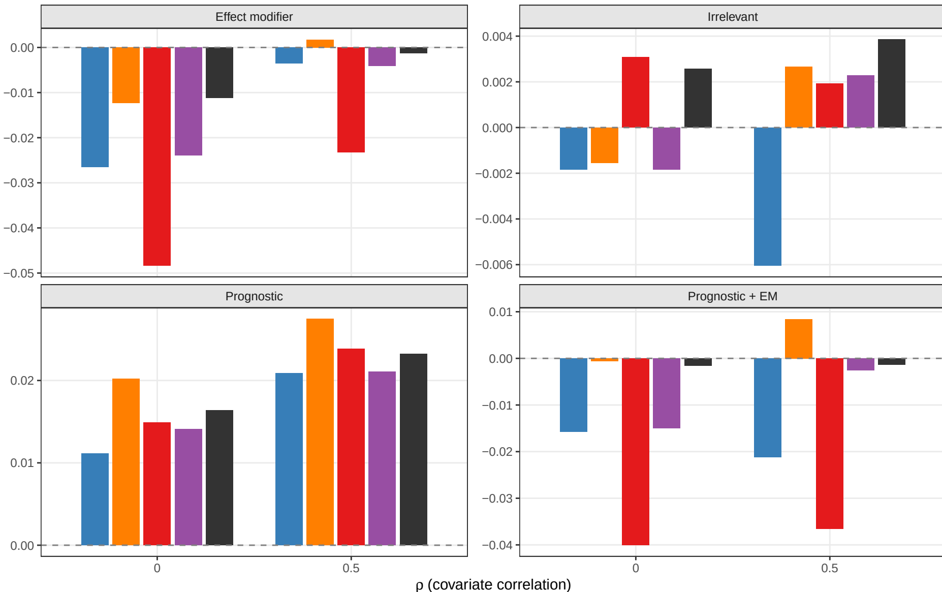
Bias in average treatment effect
