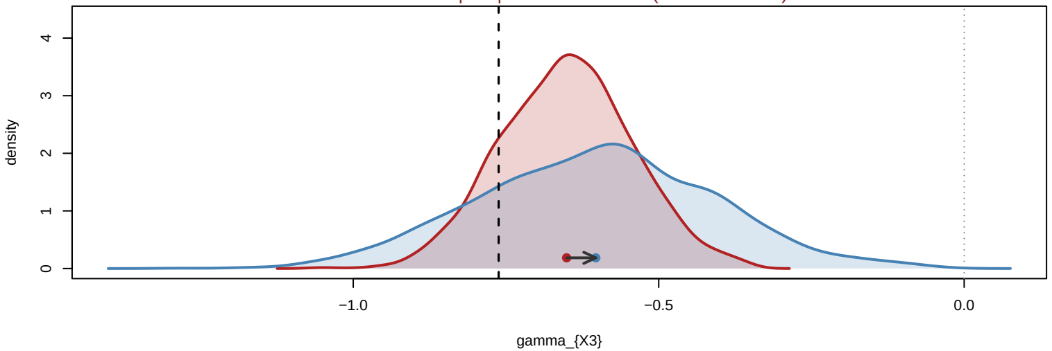
shift = +0.048 |bias|: 0.111 -> 0.159 (fusion worsens)
