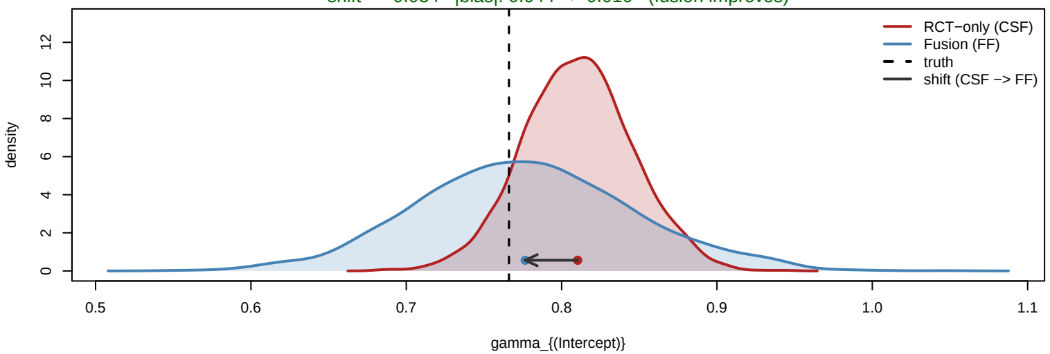
GATE projection: RCT-only vs Fusion shift = -0.034 |bias|: 0.044 -> 0.010 (fusion improves)
