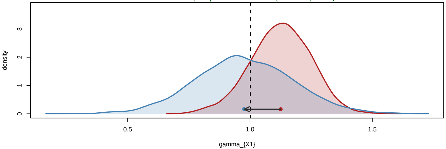
shift = -0.149 |bias|: 0.124 -> 0.025 (fusion improves)
