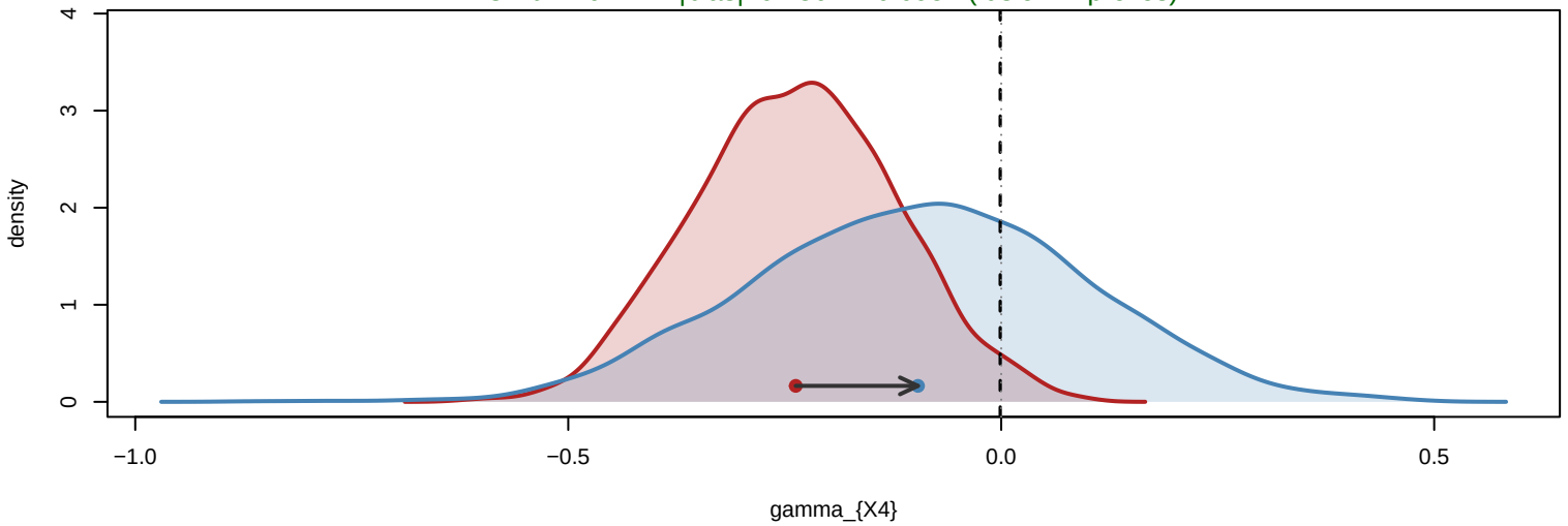
shift = +0.141 |bias|: 0.236 -> 0.095 (fusion improves)
