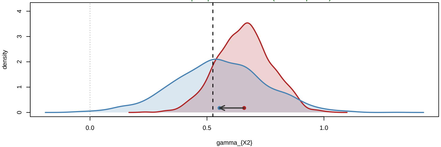
shift = -0.105 |bias|: 0.134 -> 0.028 (fusion improves)
